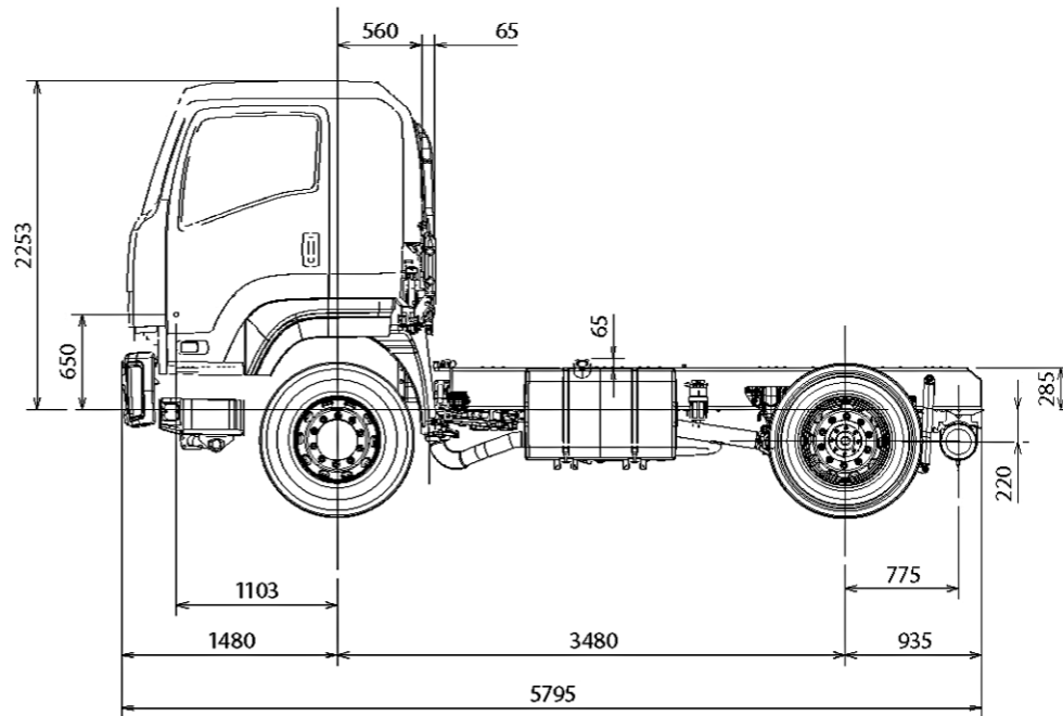
2008 Isuzu FH GXD Prime Mover
