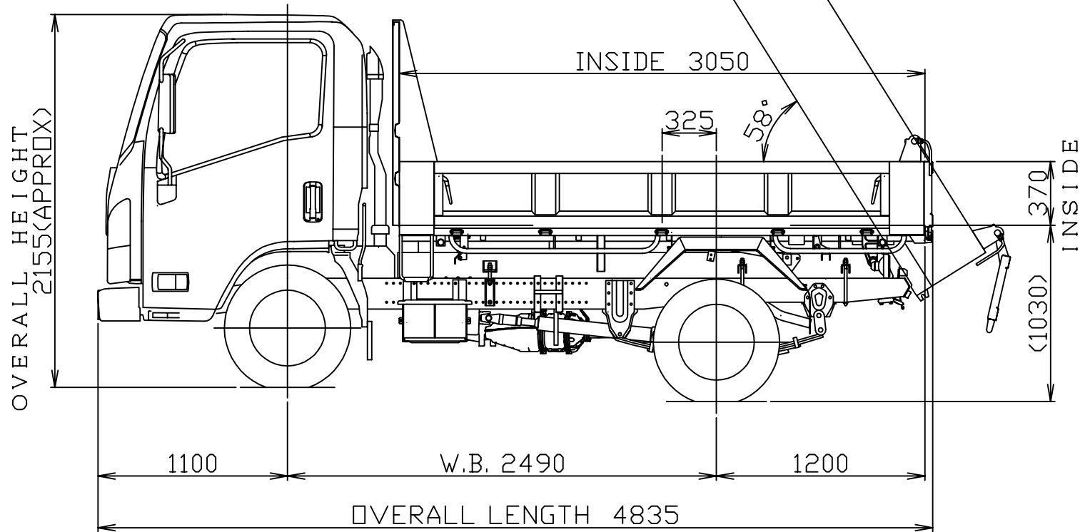
NH 2011MY Isuzu NLR 275 tipper
